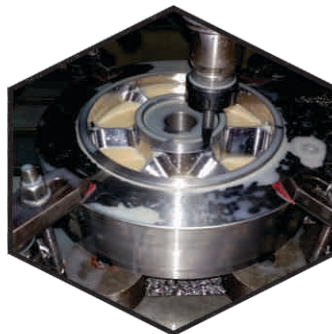
SPIDER
